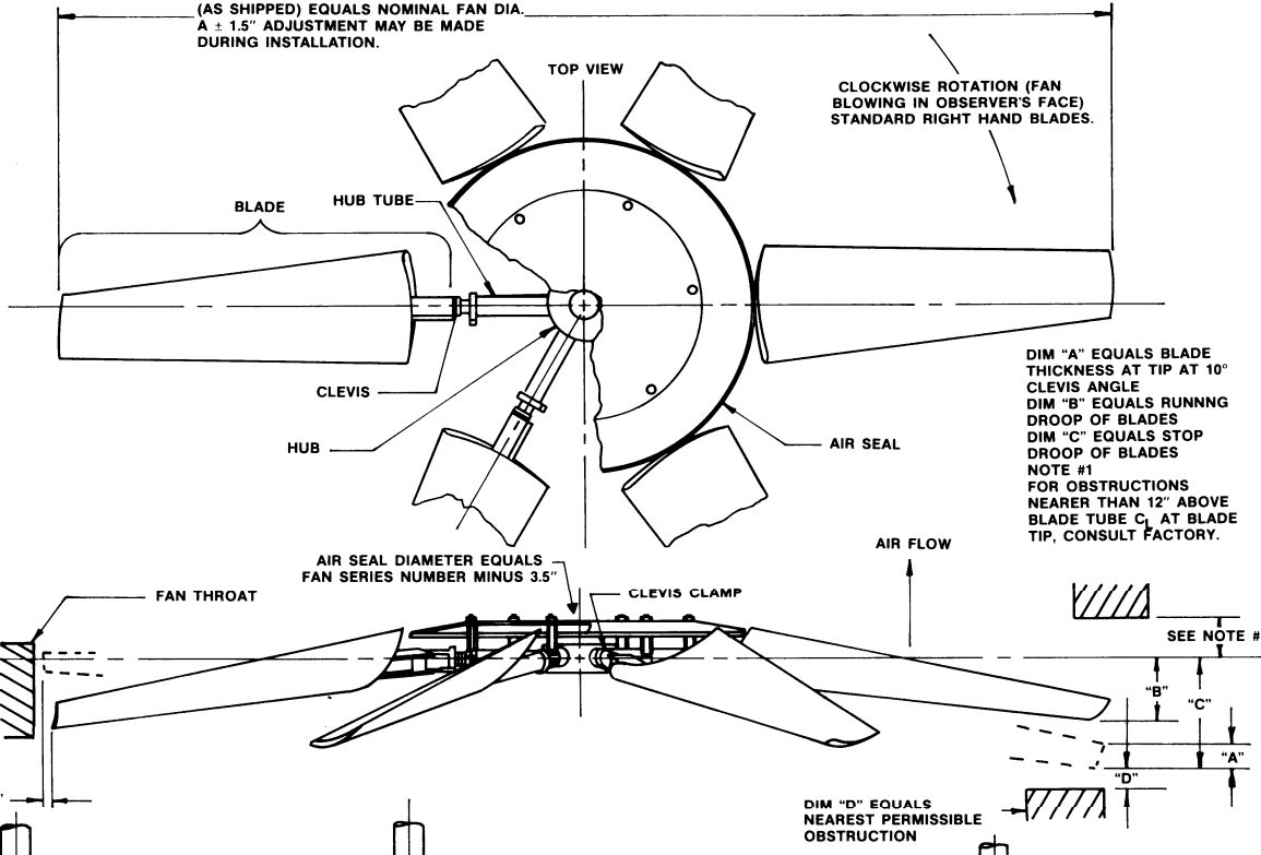
MODEL "X" EXTENDED "QD" BUSHING HUB
